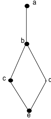
Hasse diagram for Example 3.3
