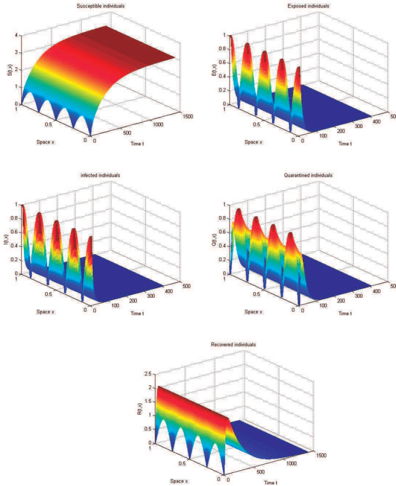
Figure 1: Spatiotemporal solution found by numerical integration of system (1.1) under conditions (1.2) and (1.3) when \mathcal{R}_0 = 0.3301
