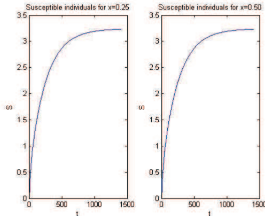
Figure 2: the curve of S in the case of x = \frac{1}{2} and x = \frac{1}{4} .
