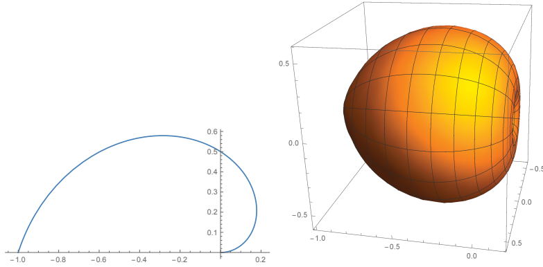
Figure 1: Curve \mathbf{f} (left) and its surface of revolution (right)
