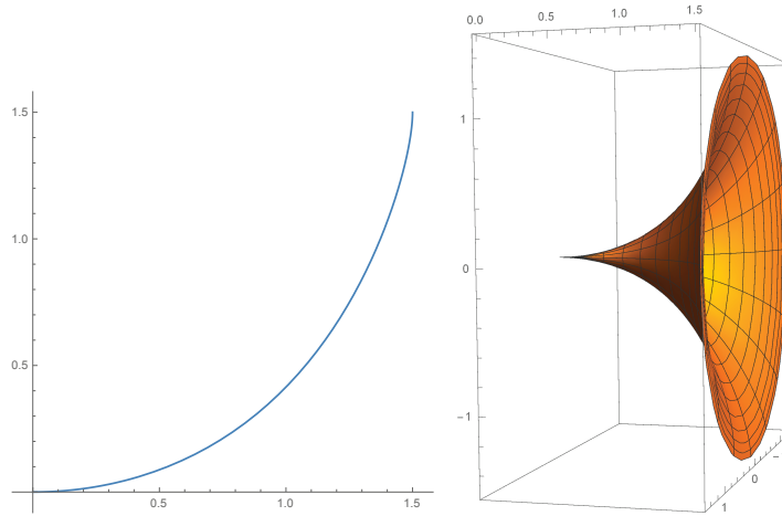
Figure 2: Curve \mathbf{g} (left) and its surface of revolution (right)
